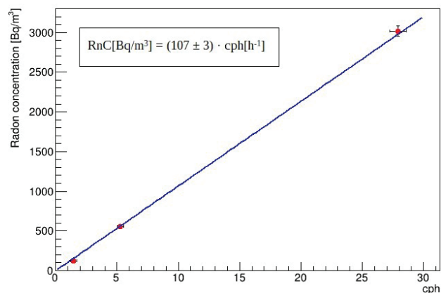
Fig. 9. Radon sensitivity of the first prototype.
